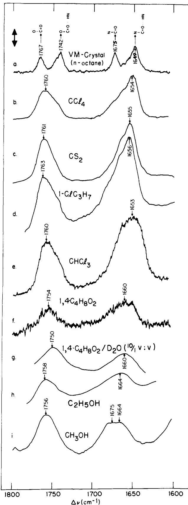
Figure 4. Comparison of Raman spectra in the \text{C}=\text{O} stretch vibration region of: (a) VM grown from n -octane, and solutions of VM dissolved in (b) \text{CCl}_4 , (c) \text{CS}_2 , (d) 1\text{-ClC}_3\text{H}_7 , (e) \text{CHCl}_3 , (f) 1,4-dioxane, (g) 1,4-dioxane/ \text{D}_2\text{O} (10:1 v/v), (h) \text{C}_2\text{H}_5\text{OH} , (i) \text{CH}_3\text{OH} . Spectra were recorded with incident power 20–200 mW, exciting frequency 457.9, 488.0, 514.5 nm, spectral resolution 3 \text{cm}^{-1} , scanning speed 0.1–0.5 \text{cm}^{-1}/\text{s} . Vertical arrow represents 300 counts/s. No analyzer in scattered beam, incident light polarized. S denotes solvent peak.
